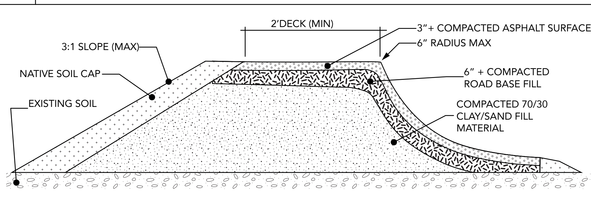
B TYPICAL BERM SURFACE CROSS-SECTION
