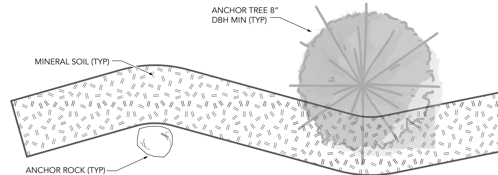
TYPICAL TRAIL BENCH CUT
