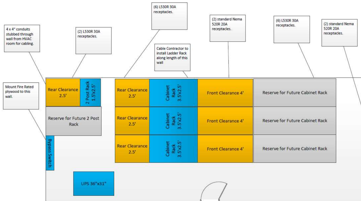
PSA 2 nd Floor Computer Room (9'x23')
